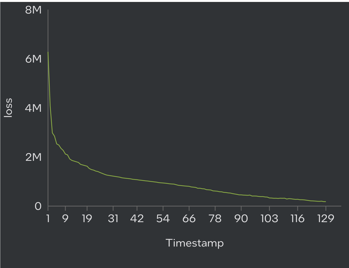
loss
