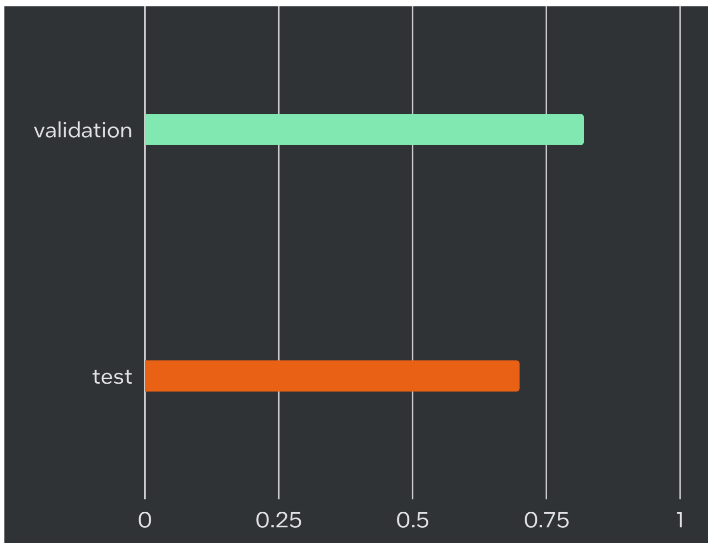
Accuracy
