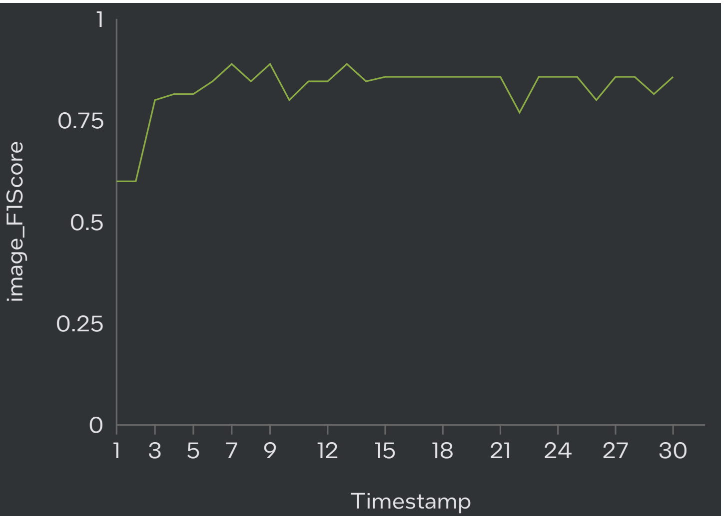
image_F1Score
